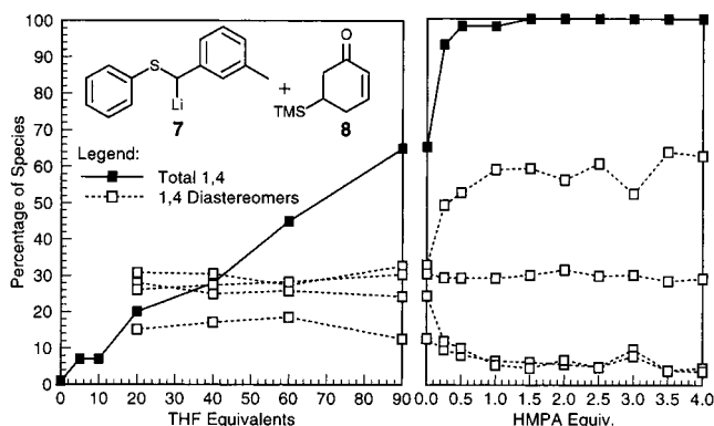
Figure 3. Changes in 1,4 addition and 1,4 diastereomer distribution as functions of the equivalents of THF in ether (left) and HMPA with 90 equiv of THF (right) for the reaction of 7 with 8 at -120\text{ }^{\circ}\text{C} in Et 2 O.
