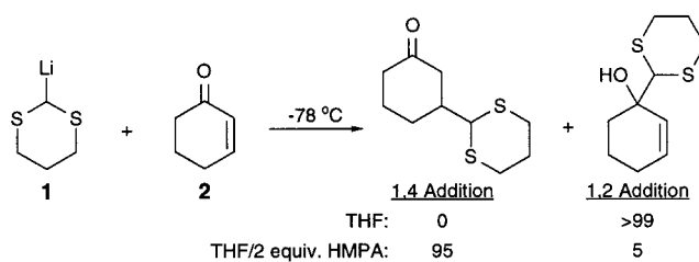
Figure 1. Demonstration of the effect of HMPA on the kinetic selectivity of enone addition. 2a
